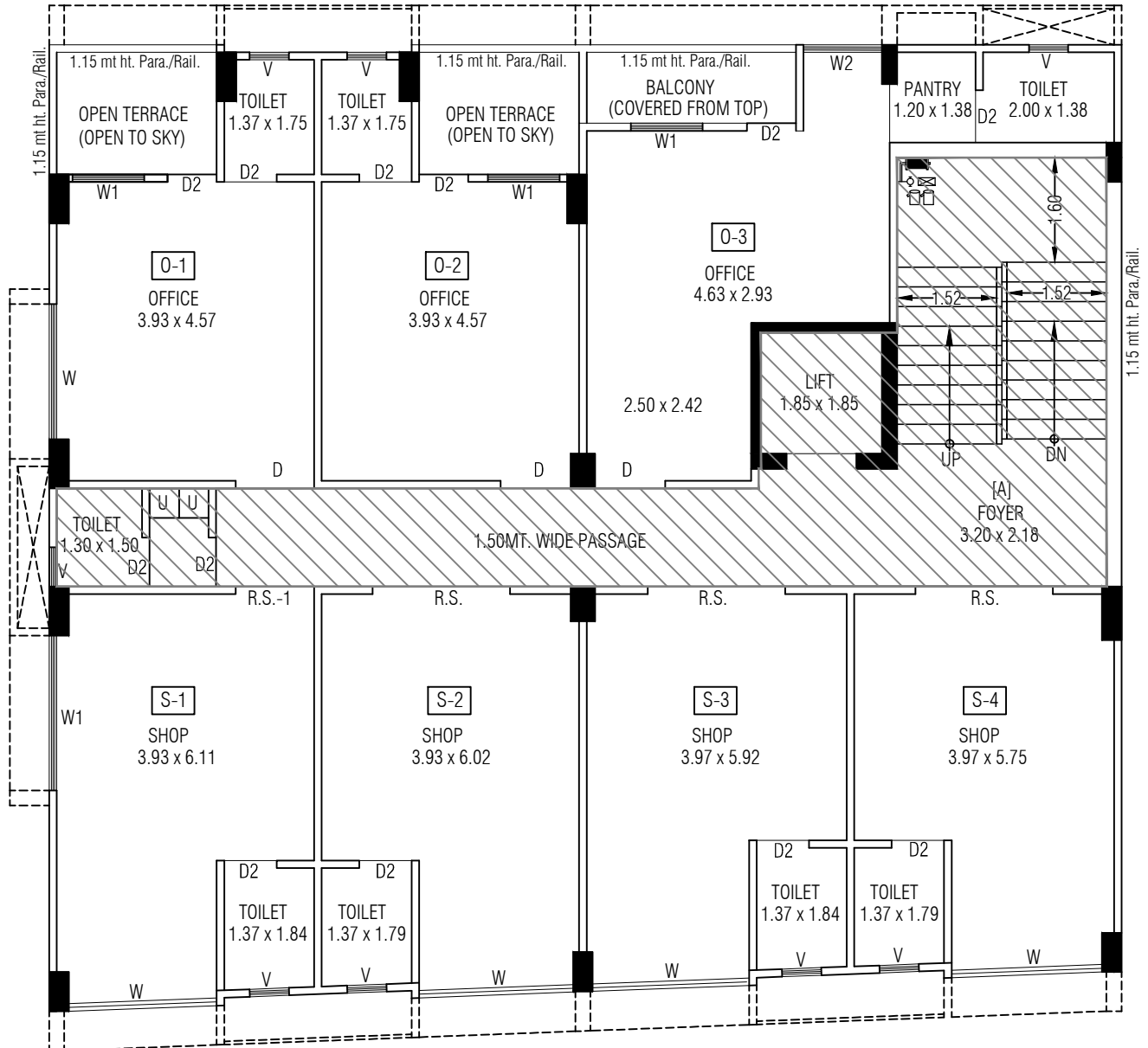
FLOOR PLAN
