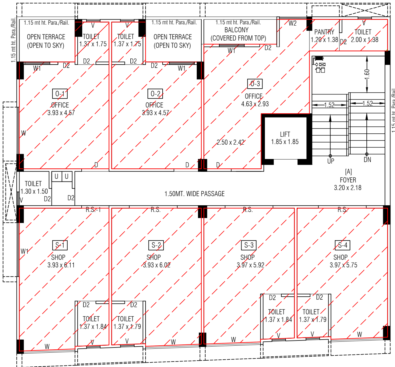
FLOOR PLAN
