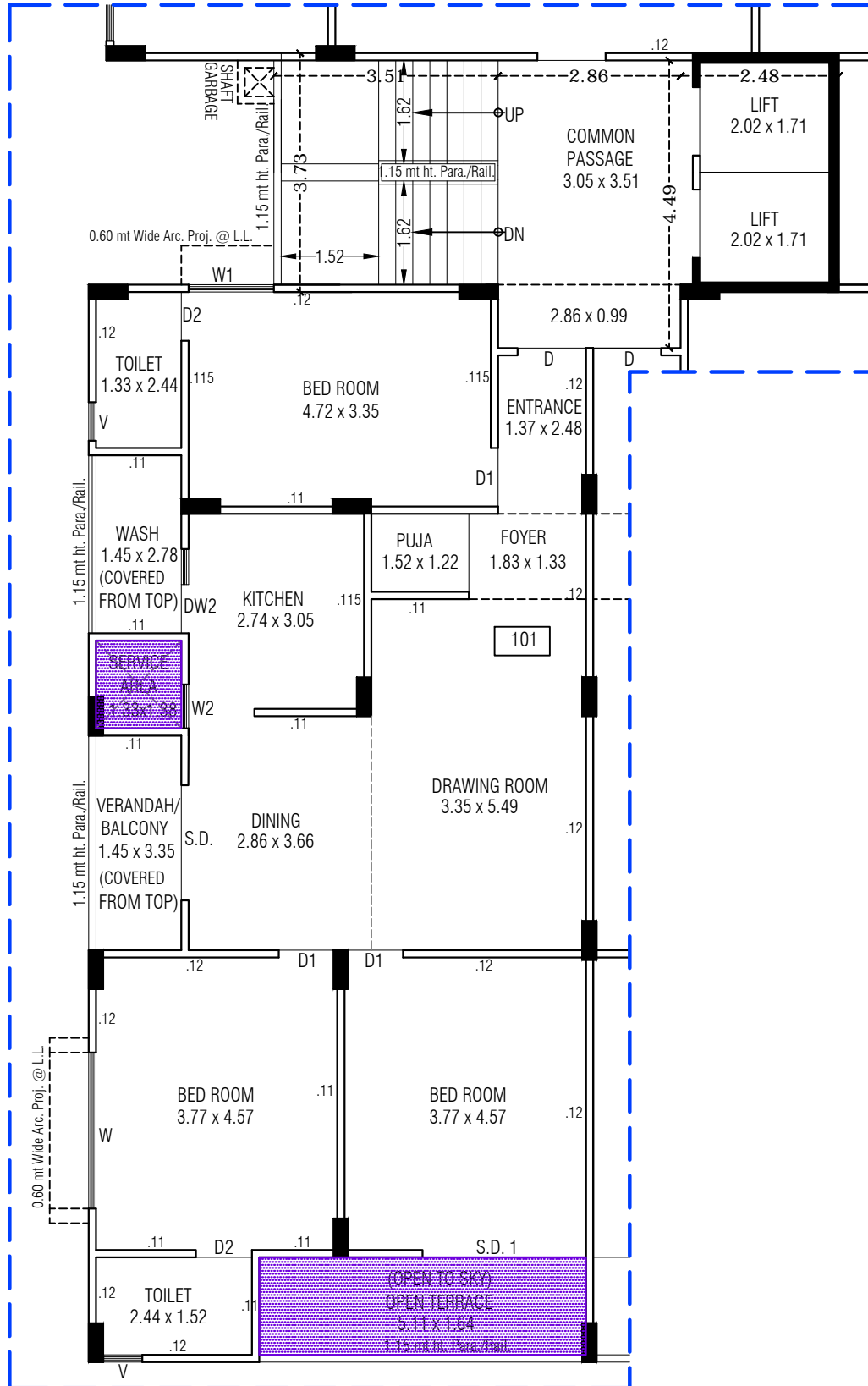
FLOOR PLAN
