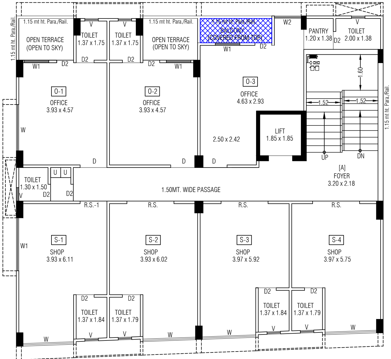
FLOOR PLAN
