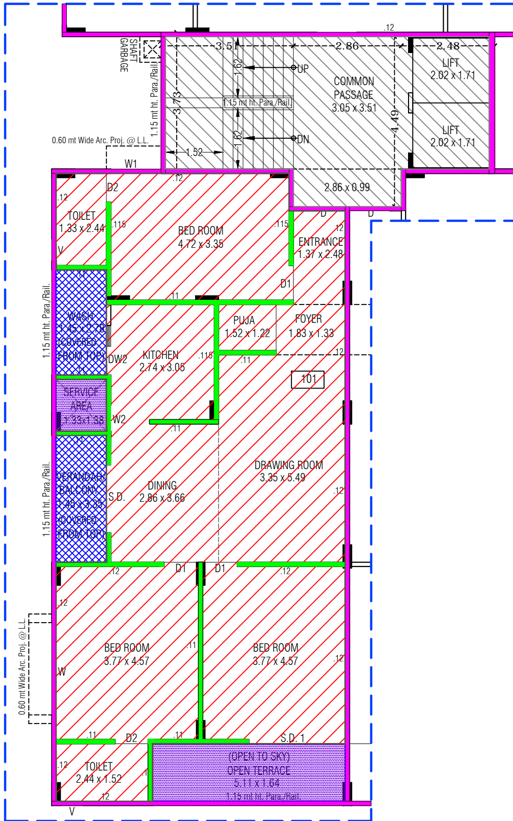
FLOOR PLAN
